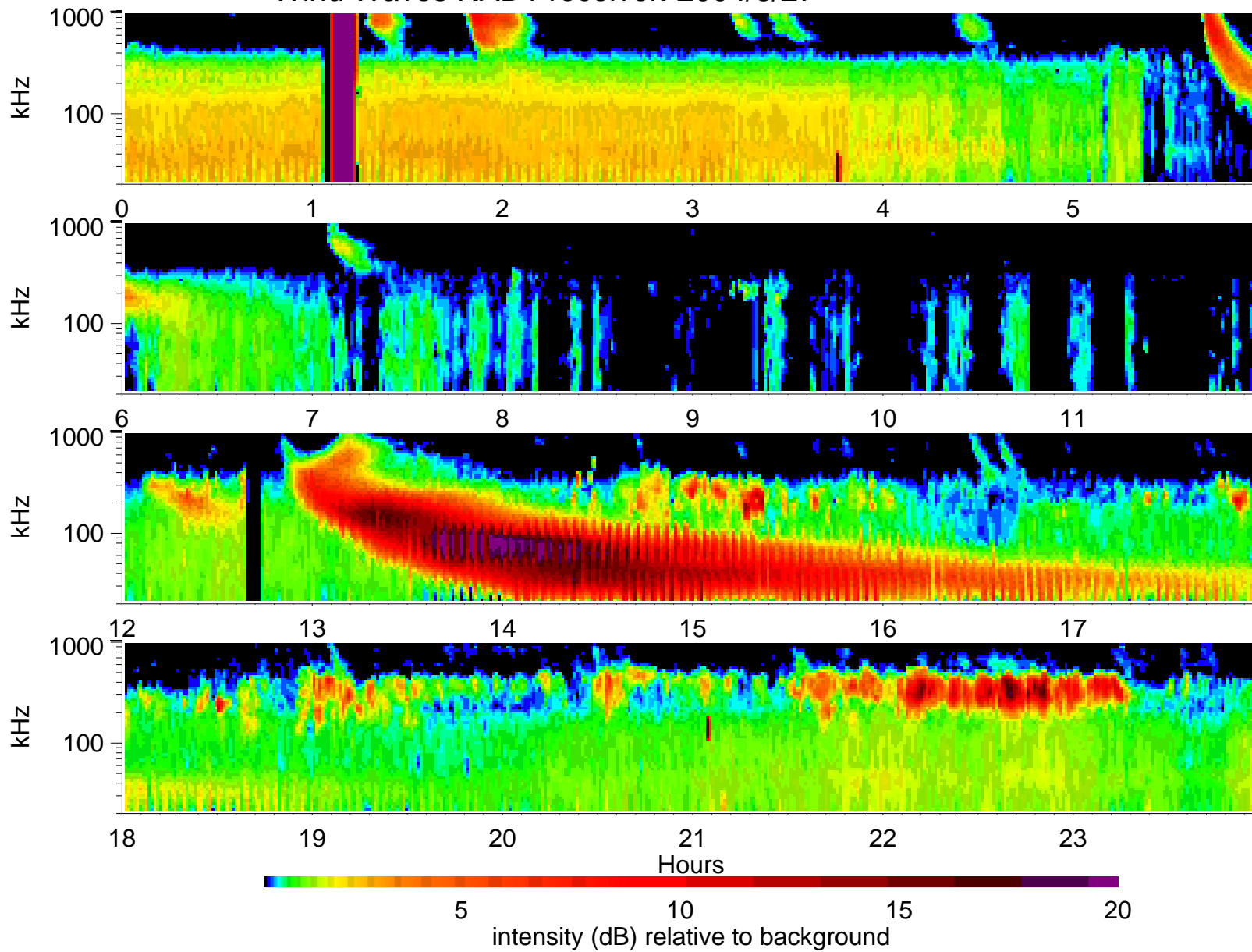
Wind Waves RAD1 receiver: 2004/8/27
