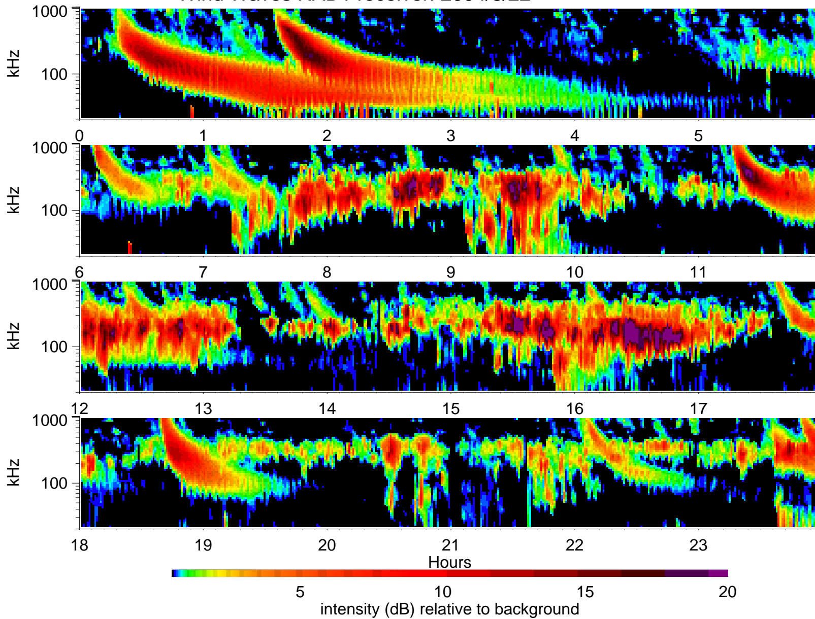
Wind Waves RAD1 receiver: 2004/8/22
