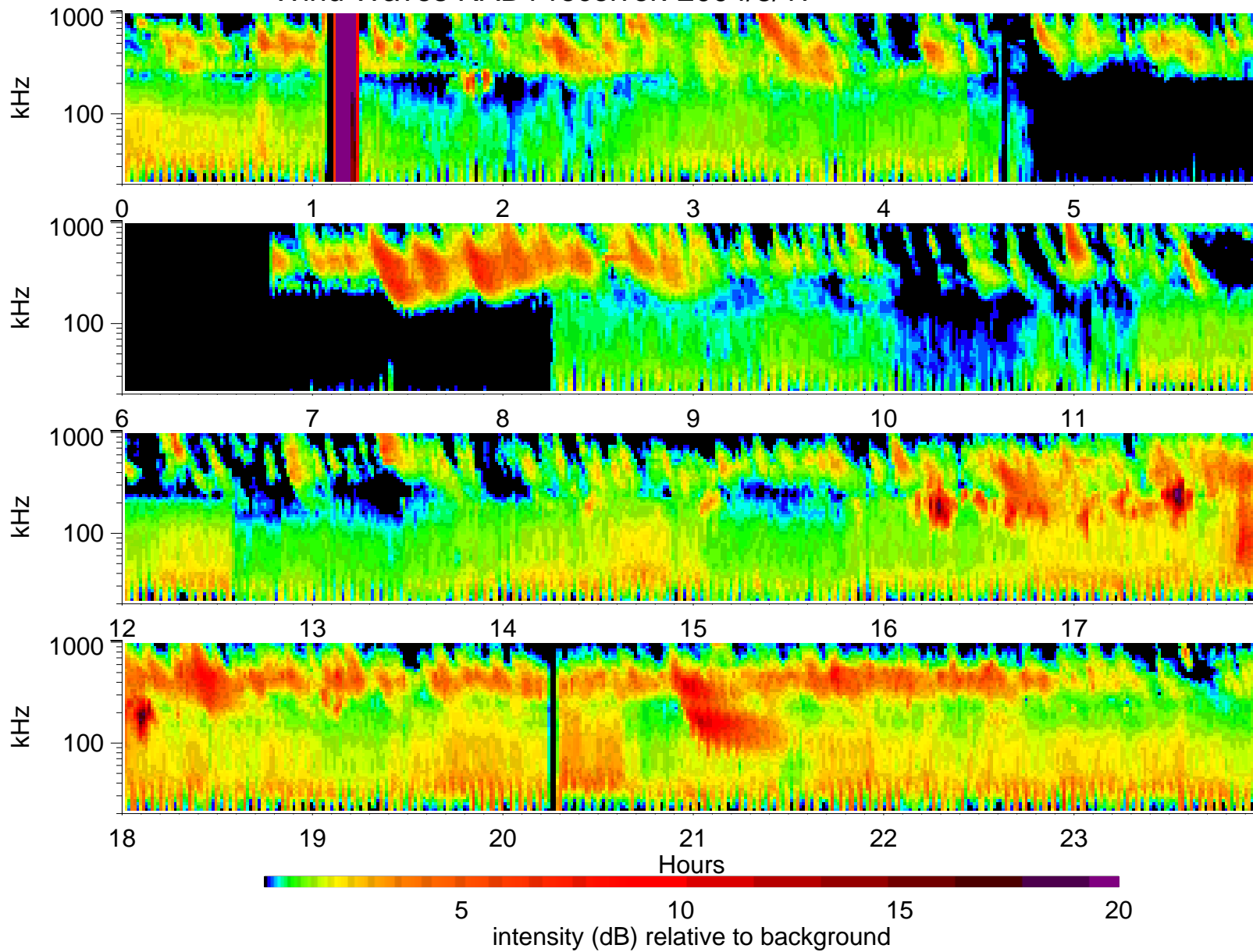
Wind Waves RAD1 receiver: 2004/8/17
