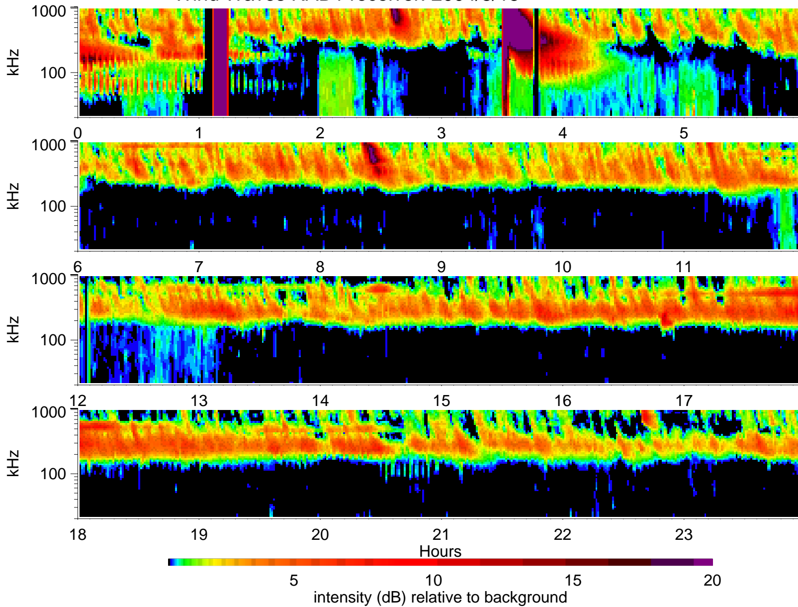
Wind Waves RAD1 receiver: 2004/8/15
