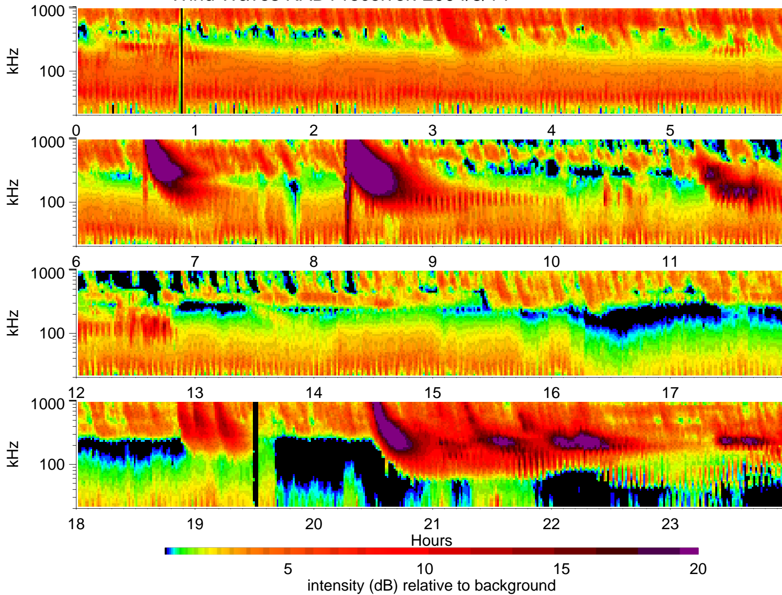
Wind Waves RAD1 receiver: 2004/8/14
