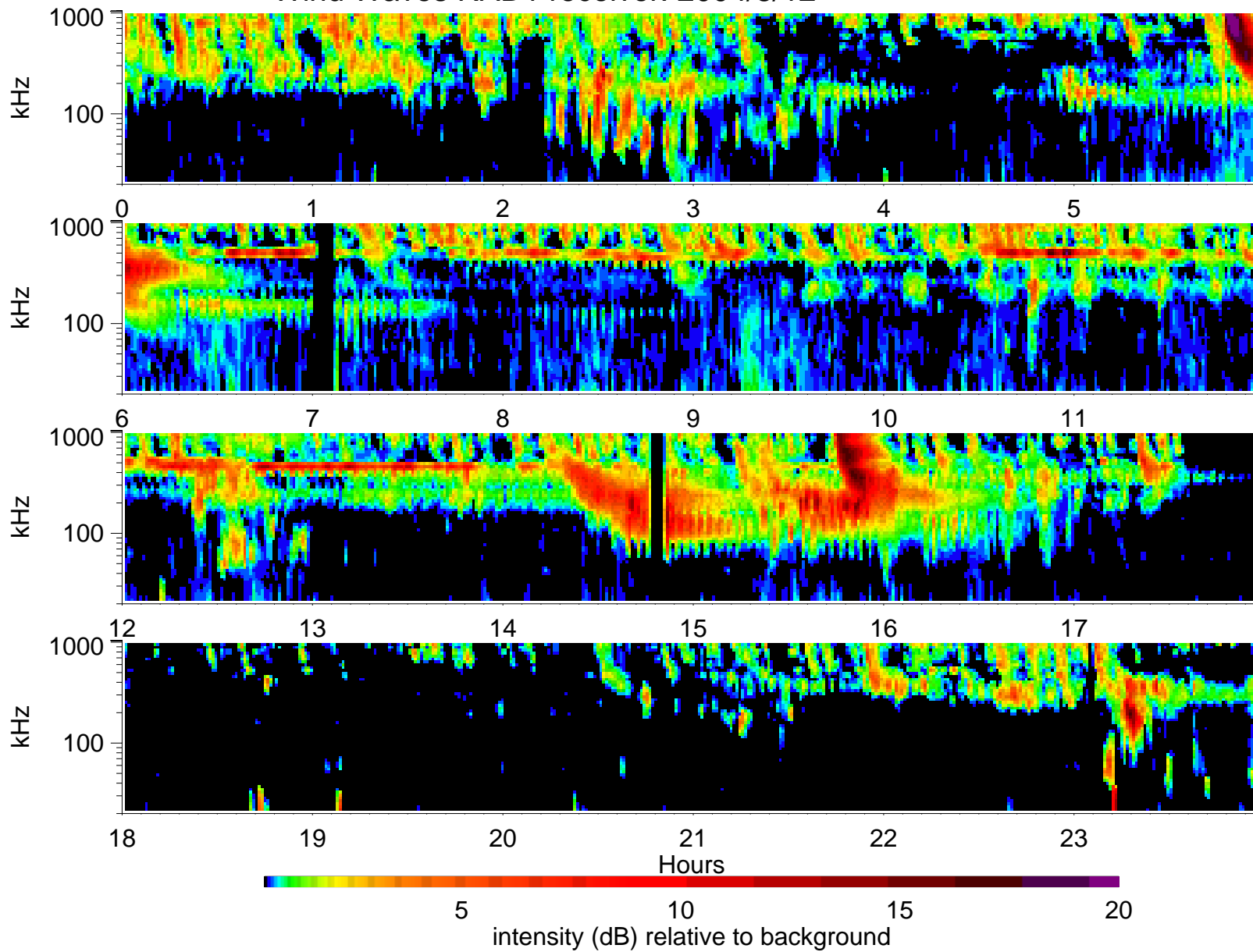
Wind Waves RAD1 receiver: 2004/8/12
