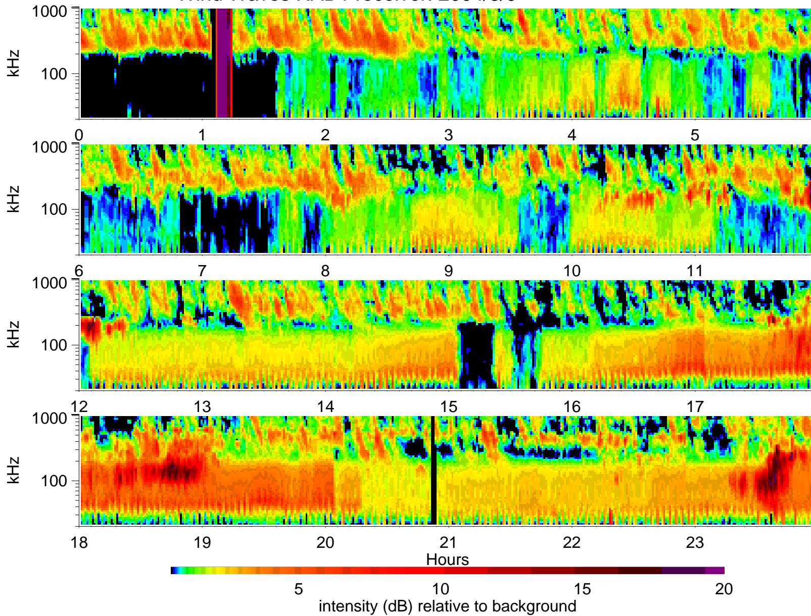
Wind Waves RAD1 receiver: 2004/8/9
