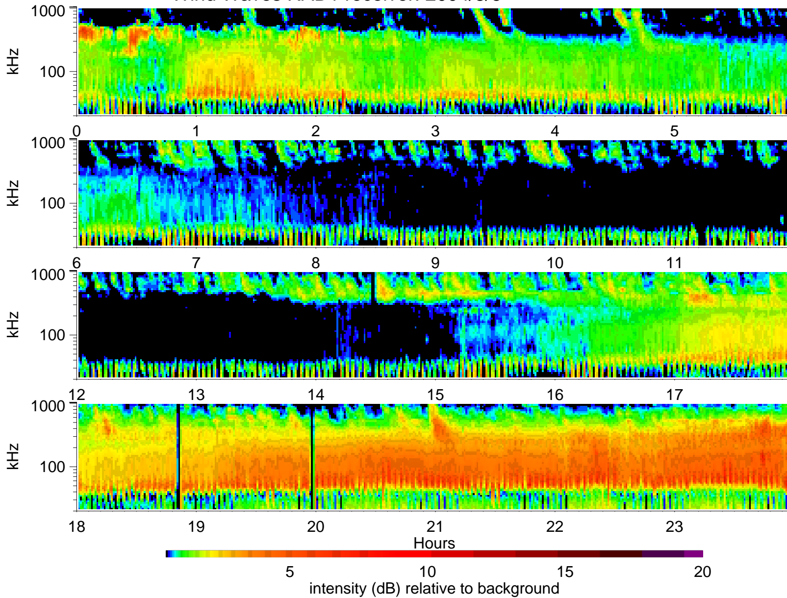
Wind Waves RAD1 receiver: 2004/8/6
