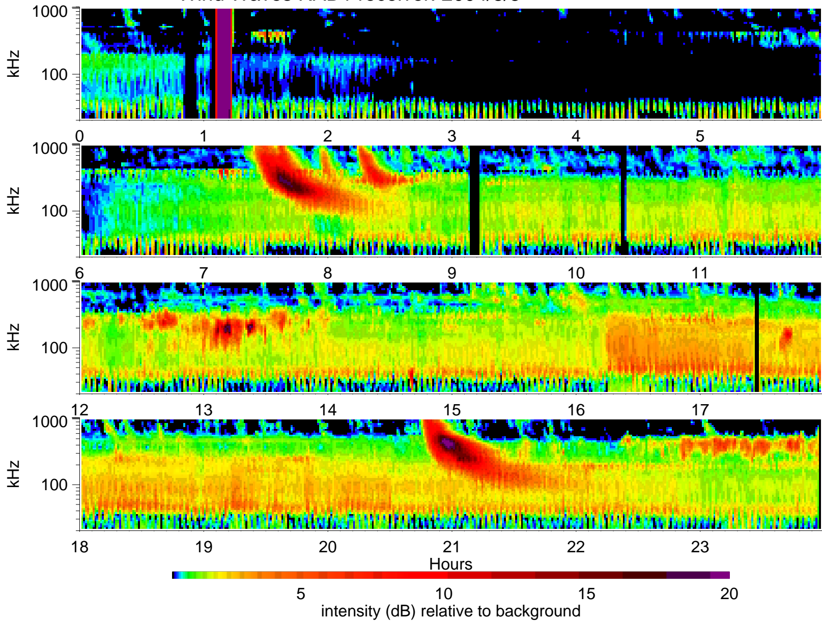
Wind Waves RAD1 receiver: 2004/8/5
