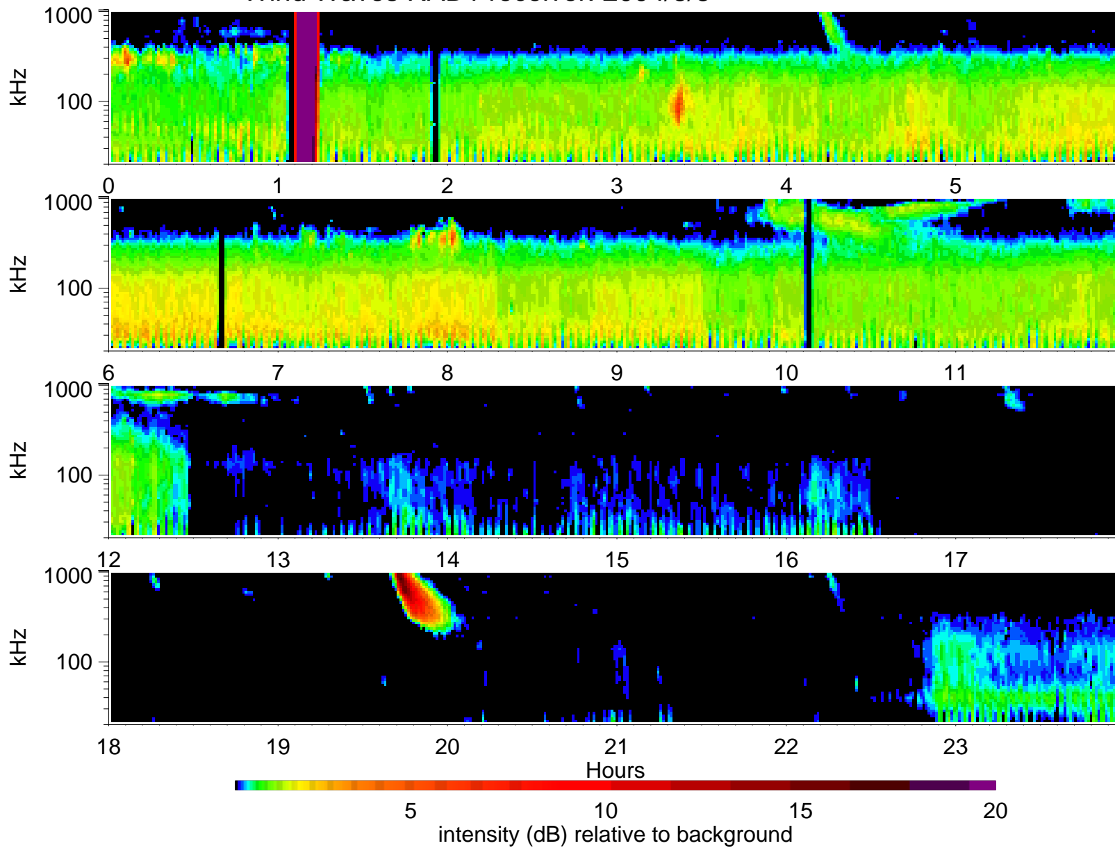
Wind Waves RAD1 receiver: 2004/8/3
