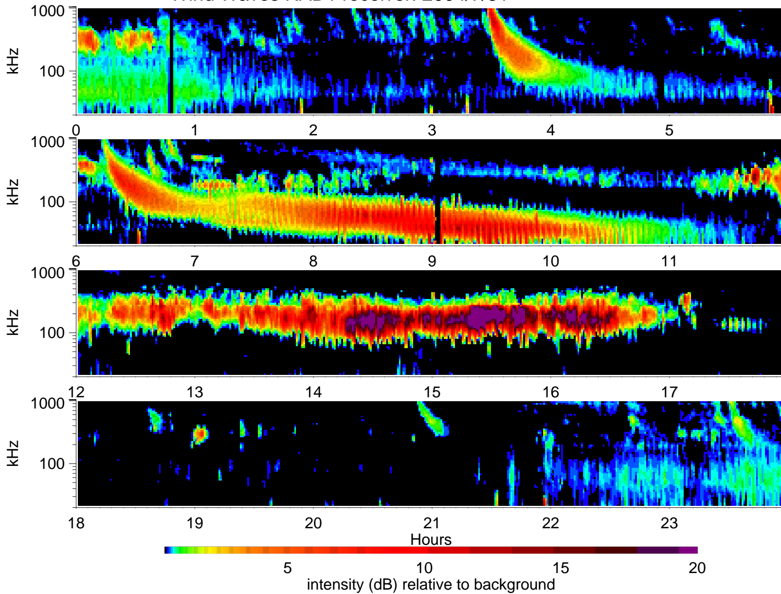
Wind Waves RAD1 receiver: 2004/7/31
