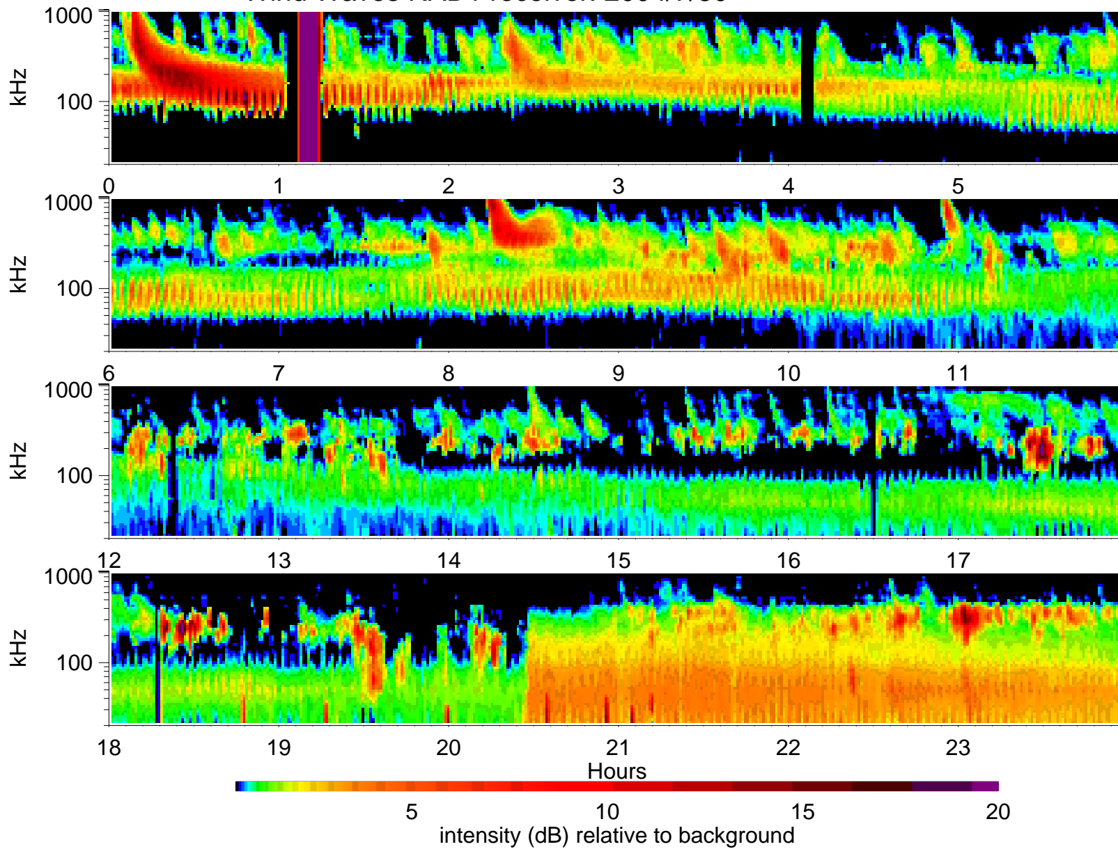
Wind Waves RAD1 receiver: 2004/7/30
