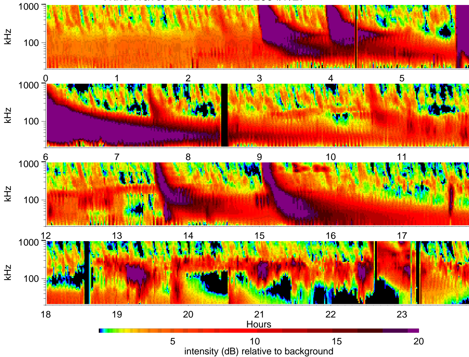
Wind Waves RAD1 receiver: 2004/7/27
