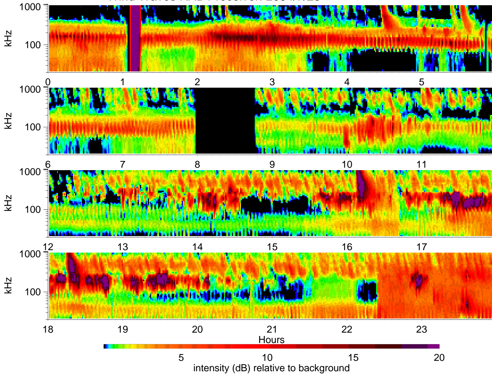
Wind Waves RAD1 receiver: 2004/7/26
