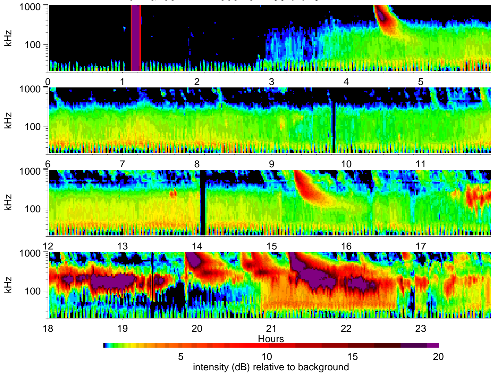
Wind Waves RAD1 receiver: 2004/7/16
