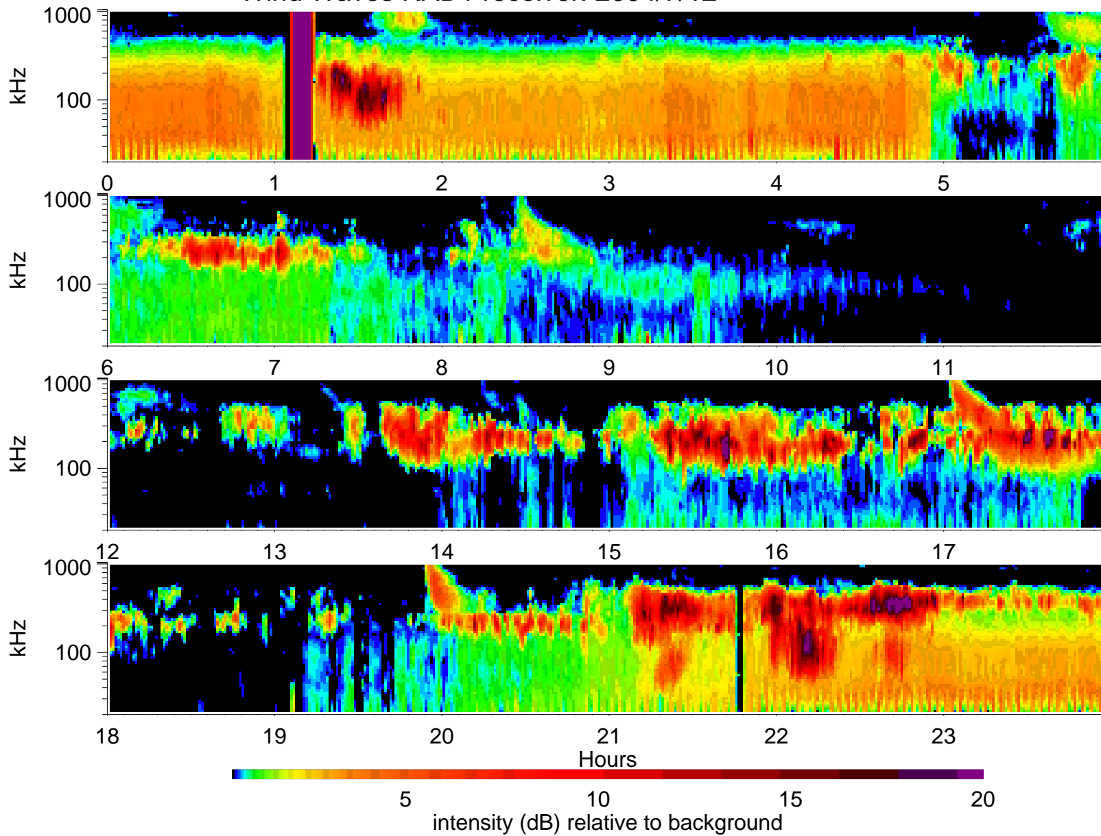
Wind Waves RAD1 receiver: 2004/7/12
