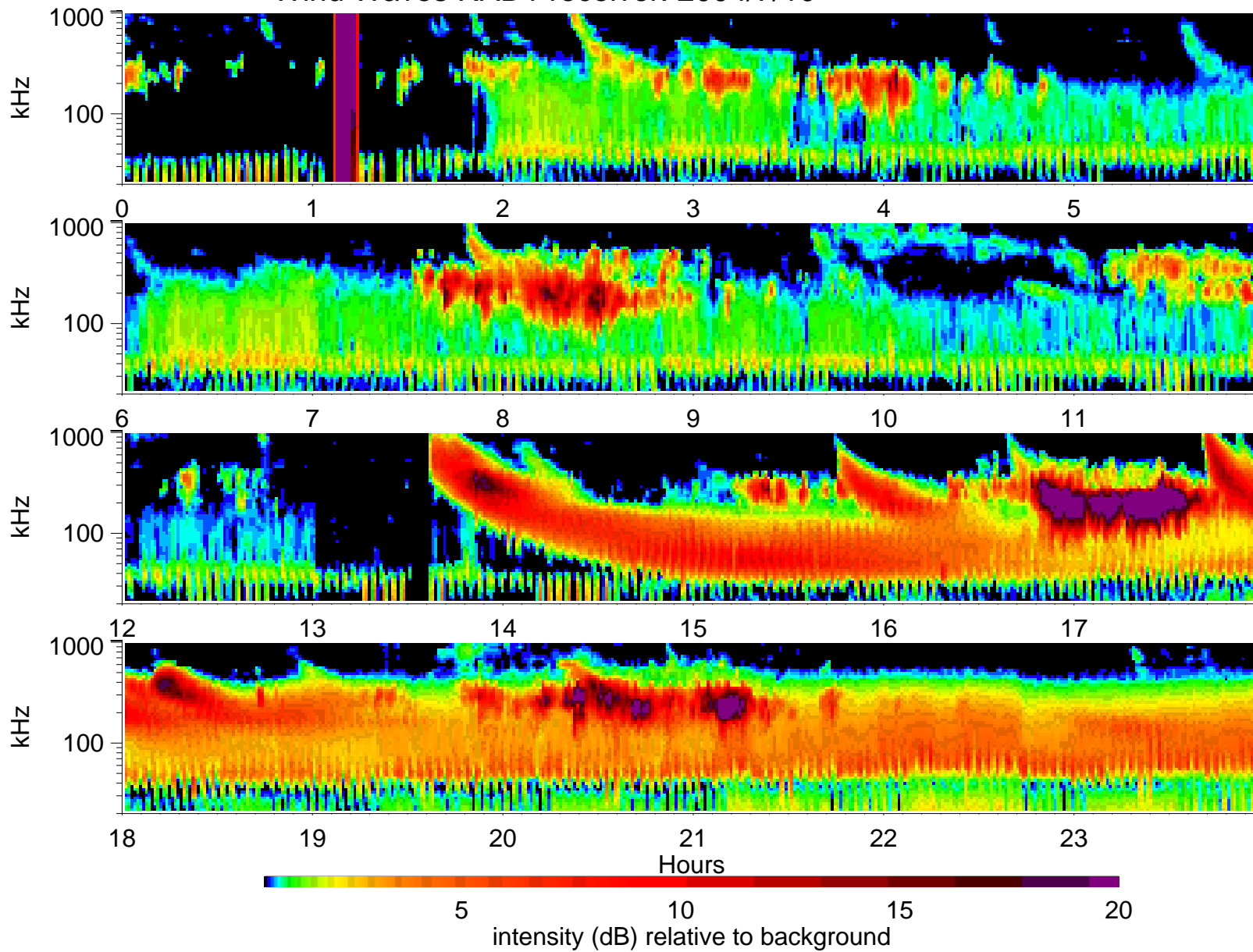
Wind Waves RAD1 receiver: 2004/7/10
