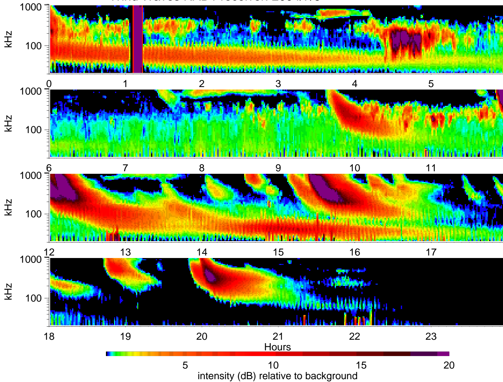
Wind Waves RAD1 receiver: 2004/7/6
