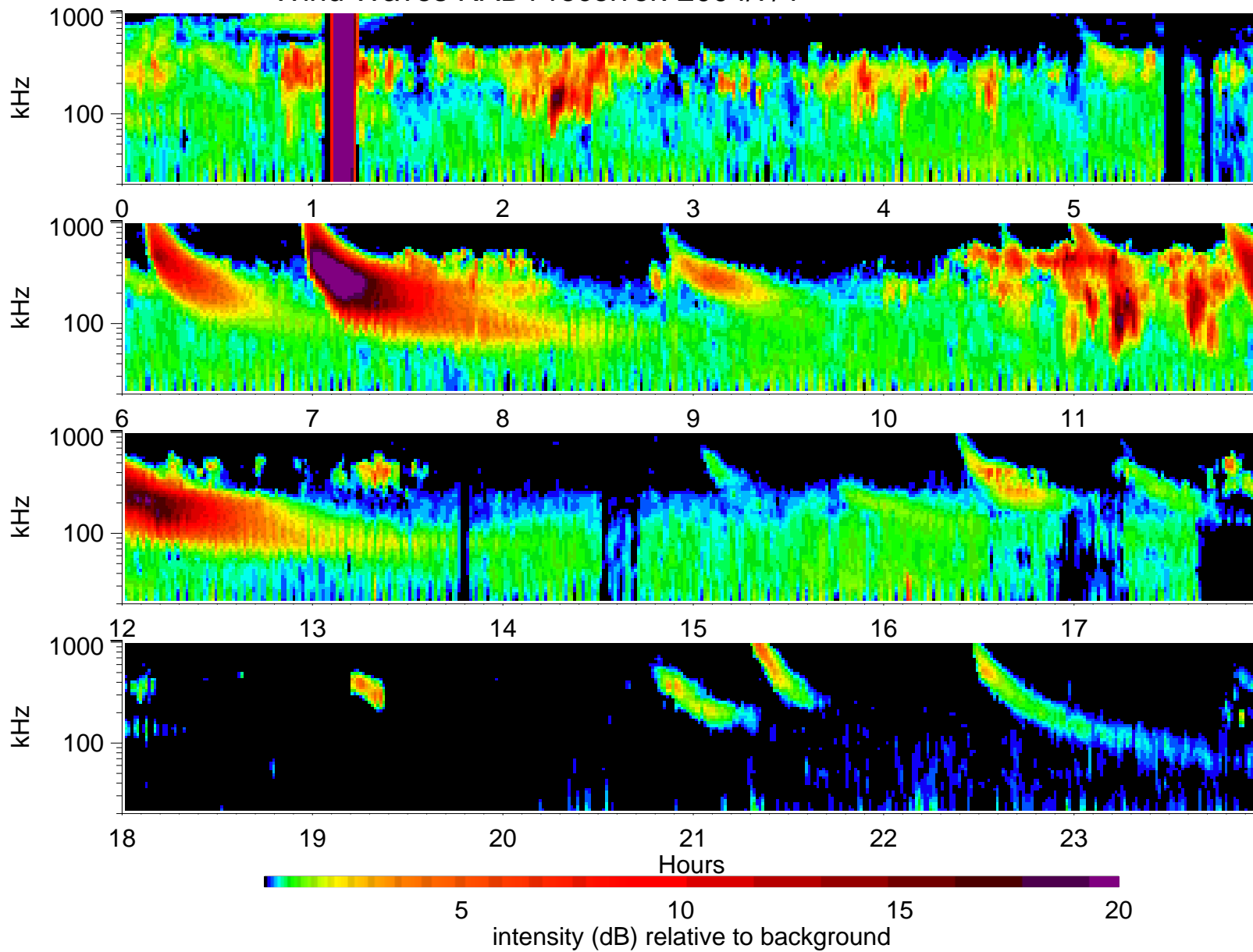
Wind Waves RAD1 receiver: 2004/7/4
