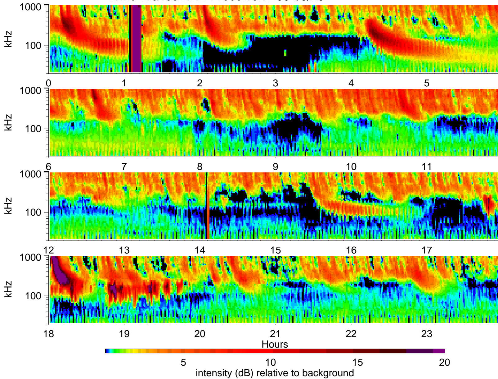
Wind Waves RAD1 receiver: 2004/6/20
