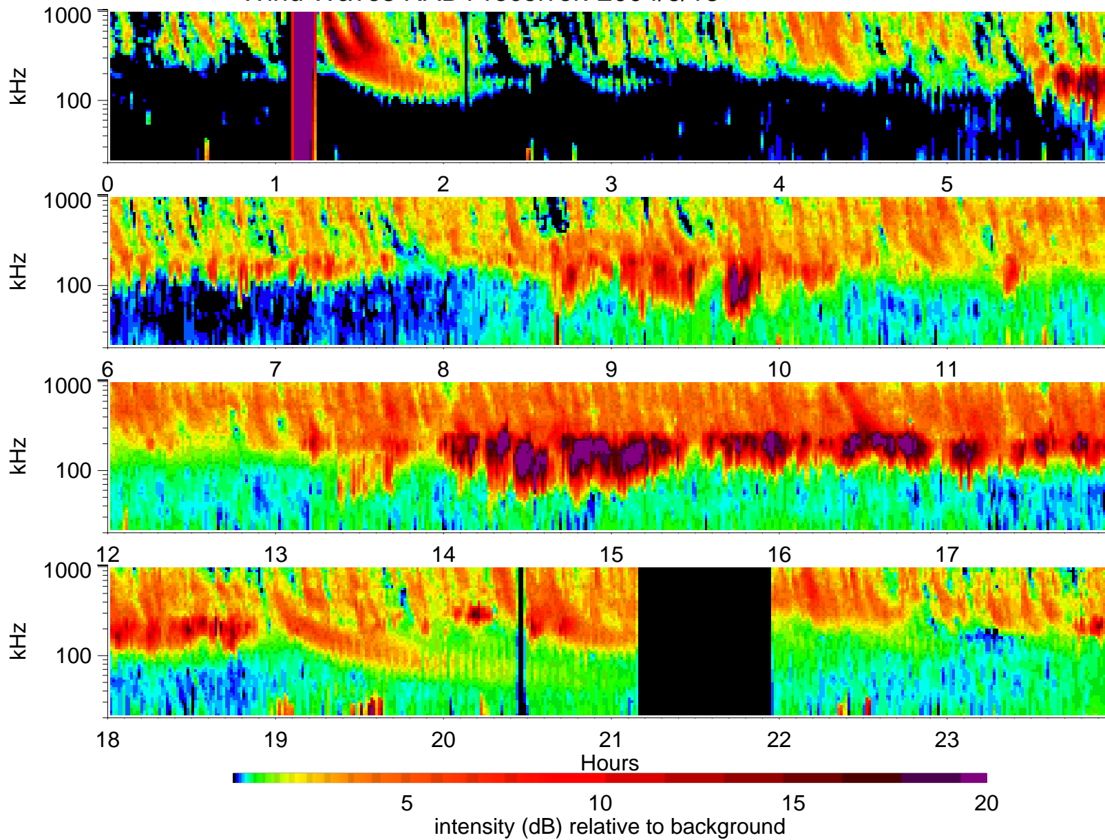
Wind Waves RAD1 receiver: 2004/6/18
