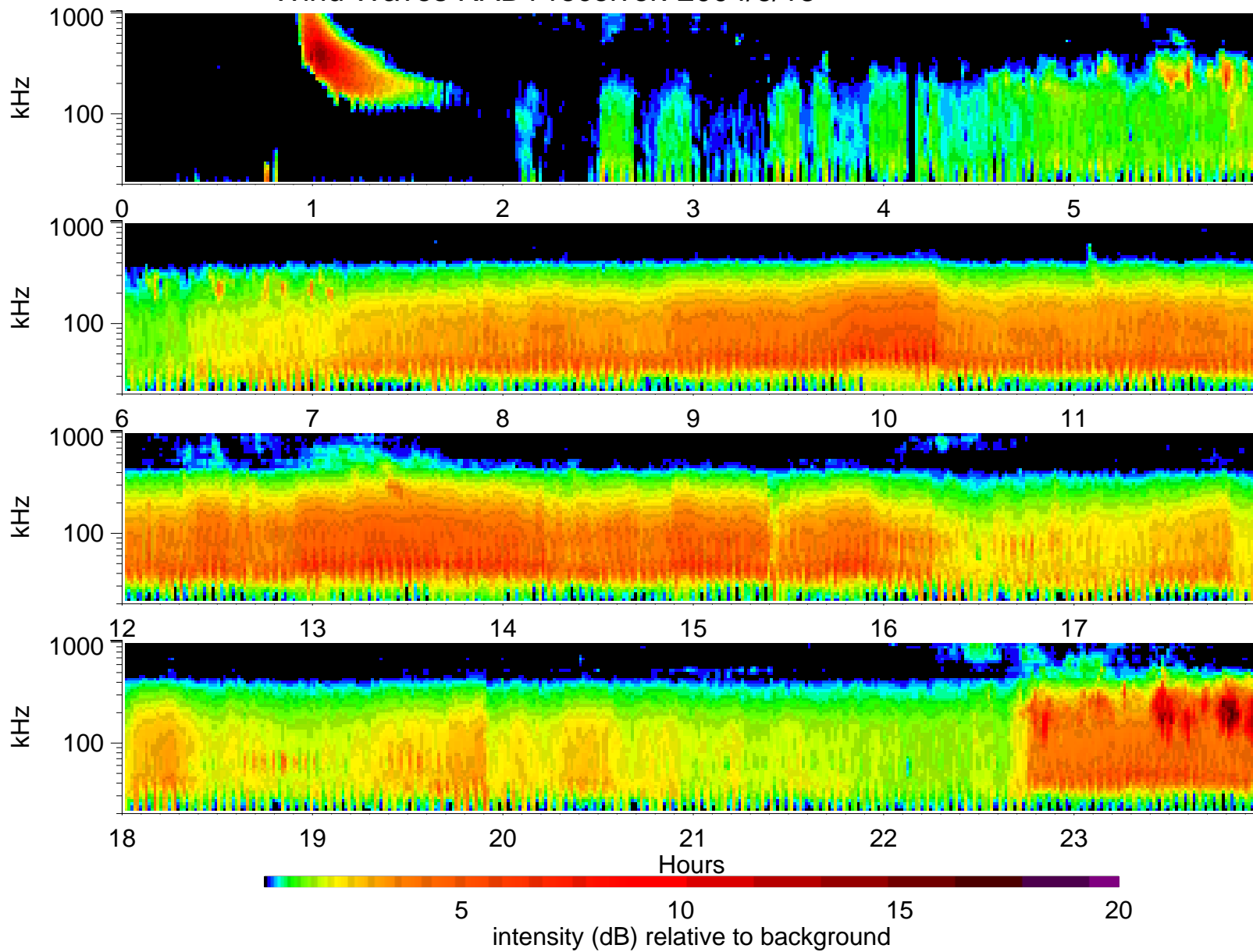
Wind Waves RAD1 receiver: 2004/6/13
