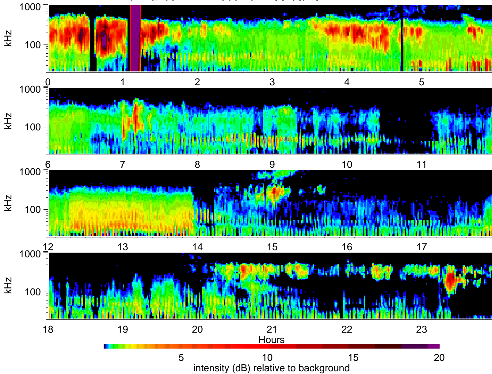
Wind Waves RAD1 receiver: 2004/6/10
