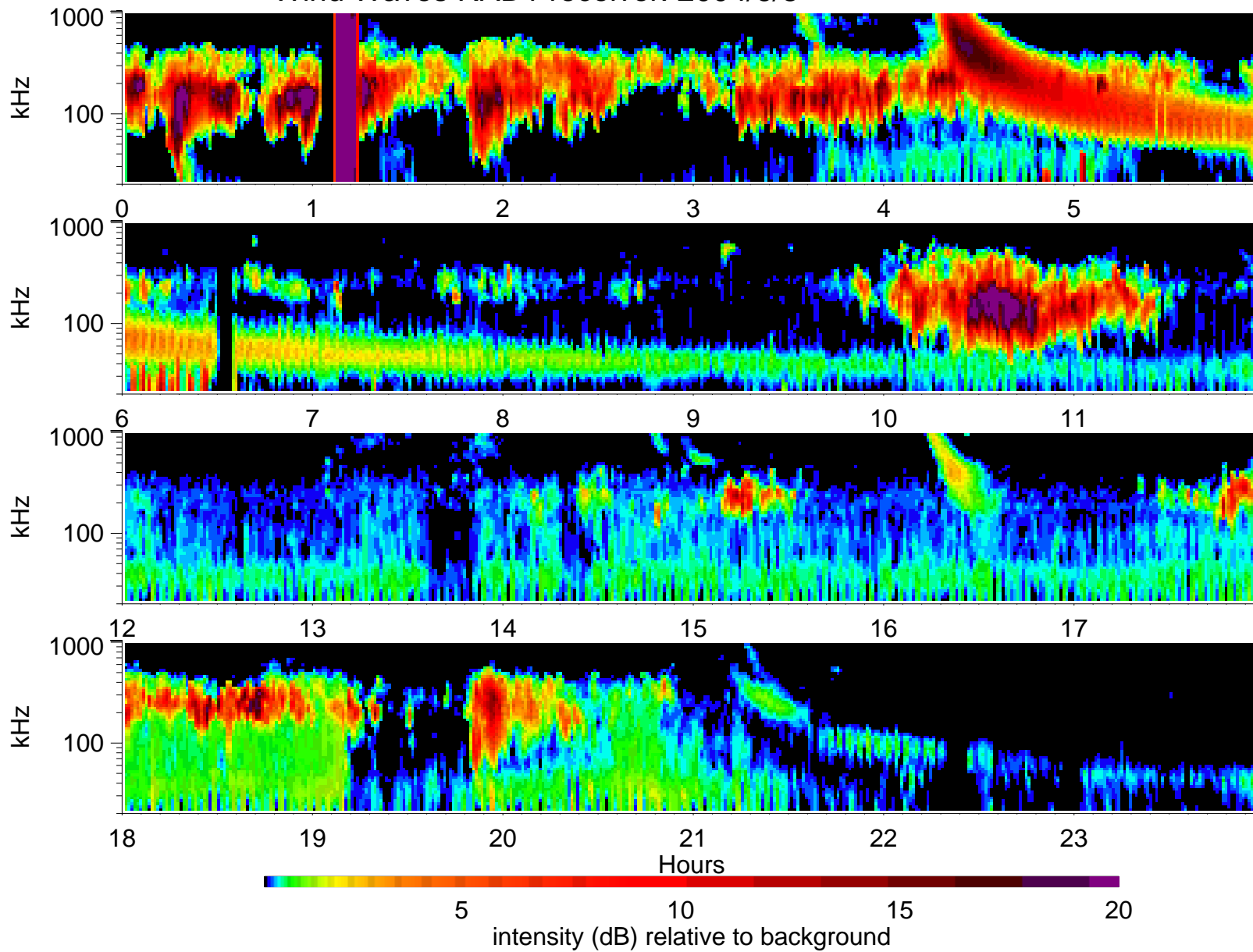
Wind Waves RAD1 receiver: 2004/6/8
