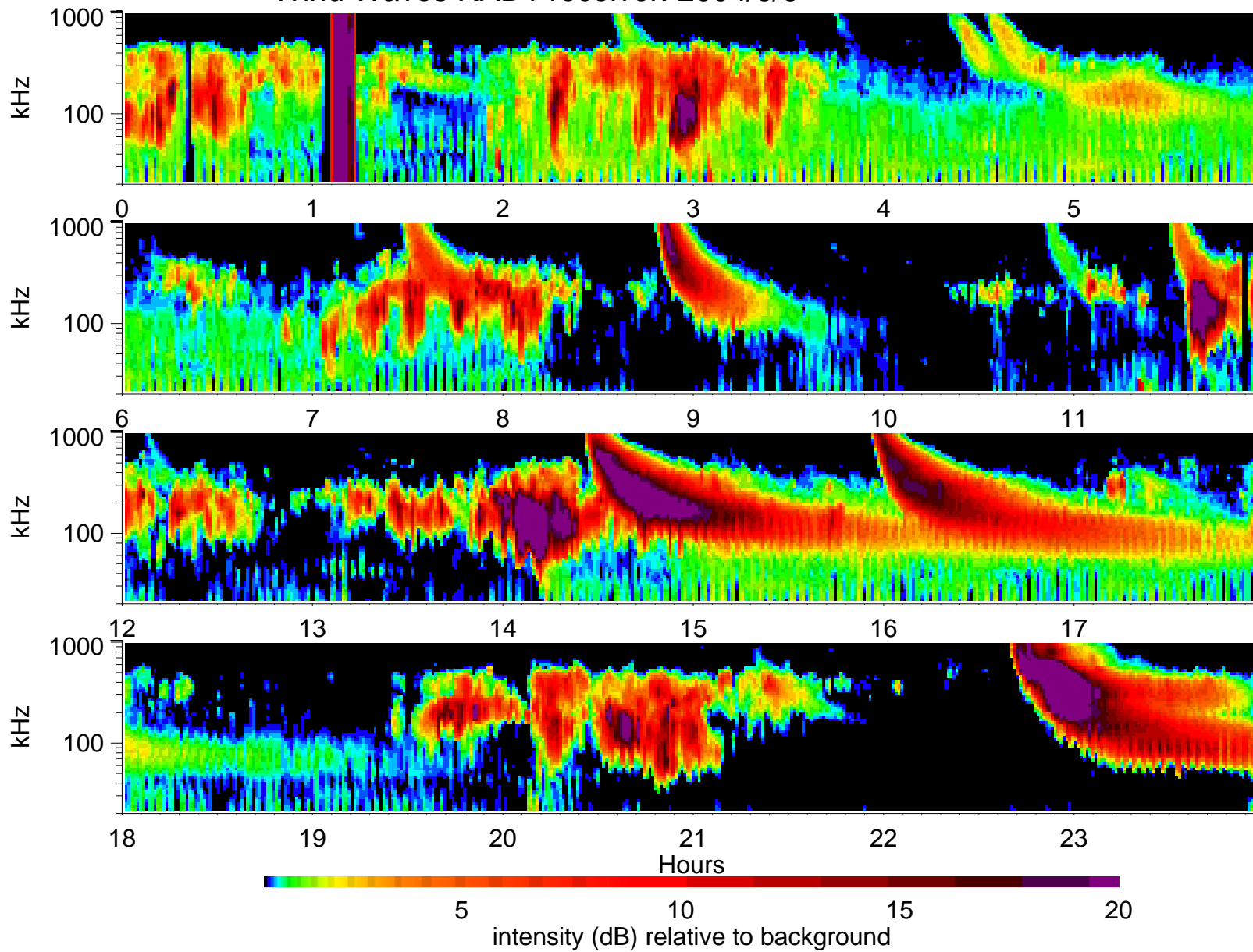
Wind Waves RAD1 receiver: 2004/6/6
