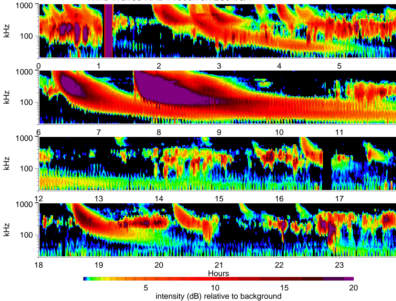
Wind Waves RAD1 receiver: 2004/6/4
