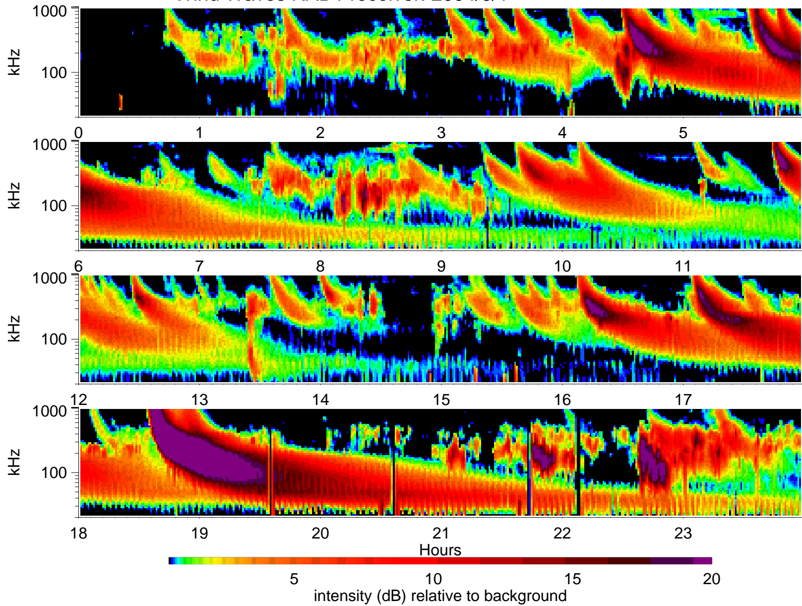
Wind Waves RAD1 receiver: 2004/6/1
