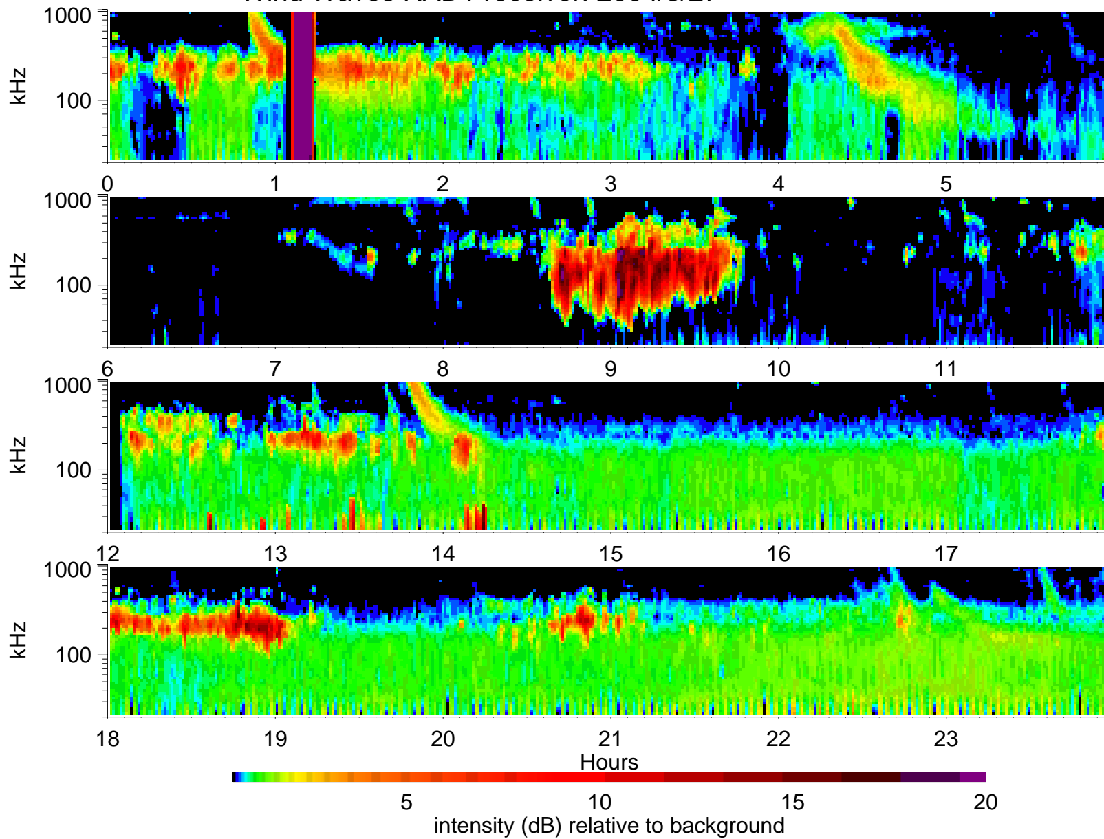
Wind Waves RAD1 receiver: 2004/5/27
