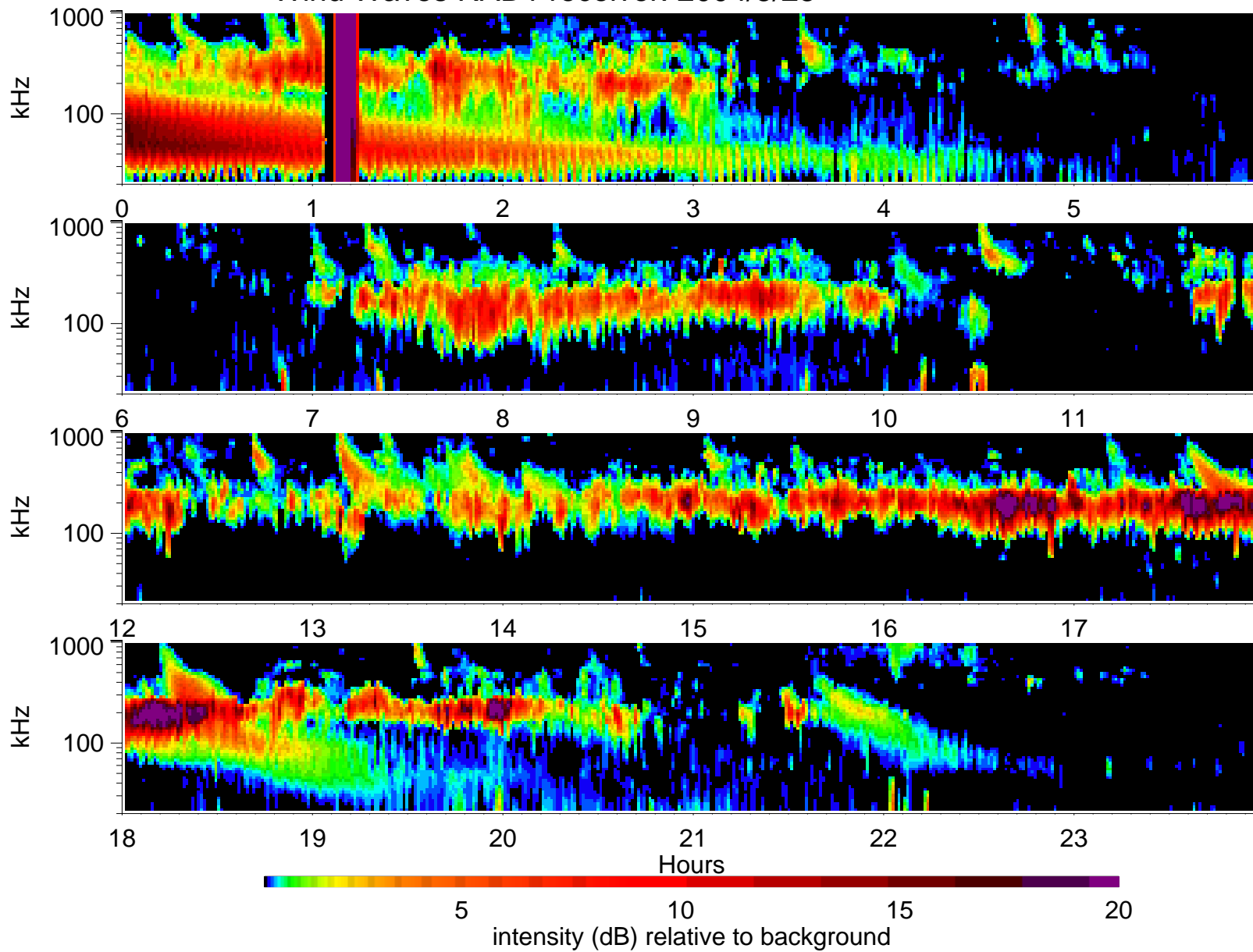
Wind Waves RAD1 receiver: 2004/5/25
