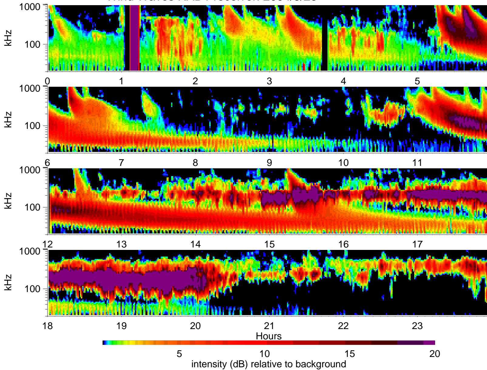
Wind Waves RAD1 receiver: 2004/5/23
