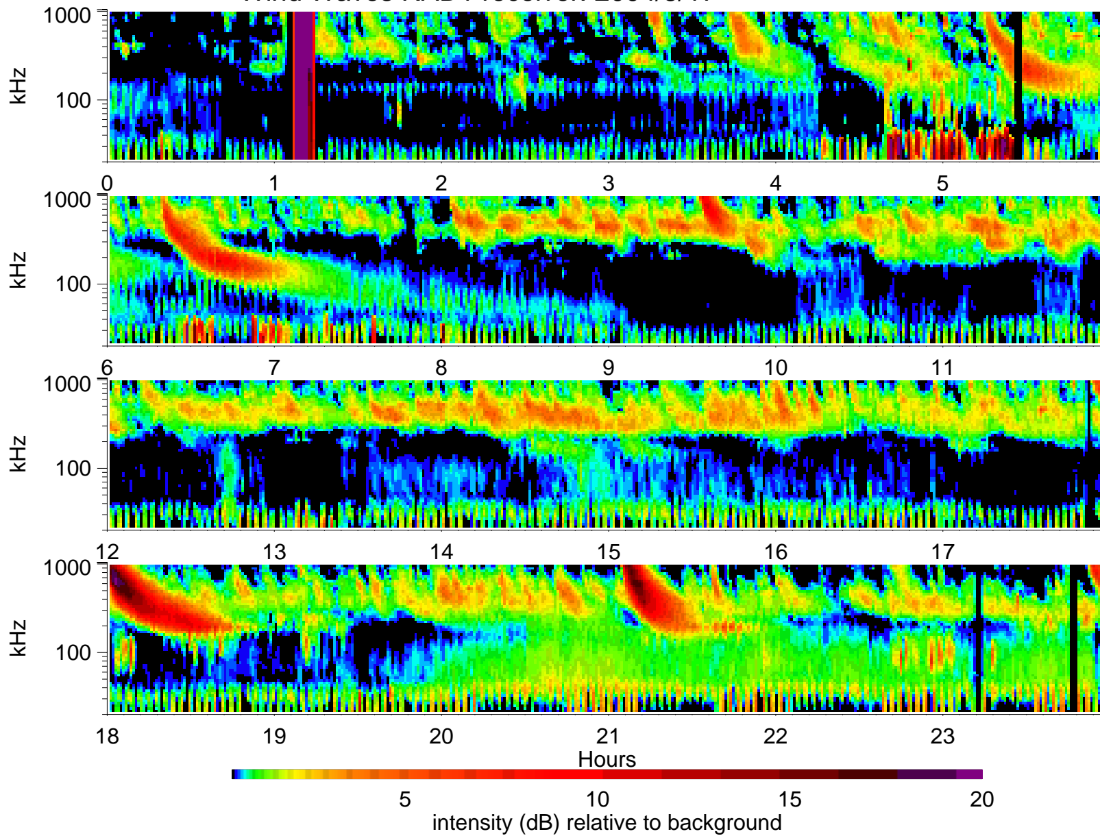
Wind Waves RAD1 receiver: 2004/5/17
