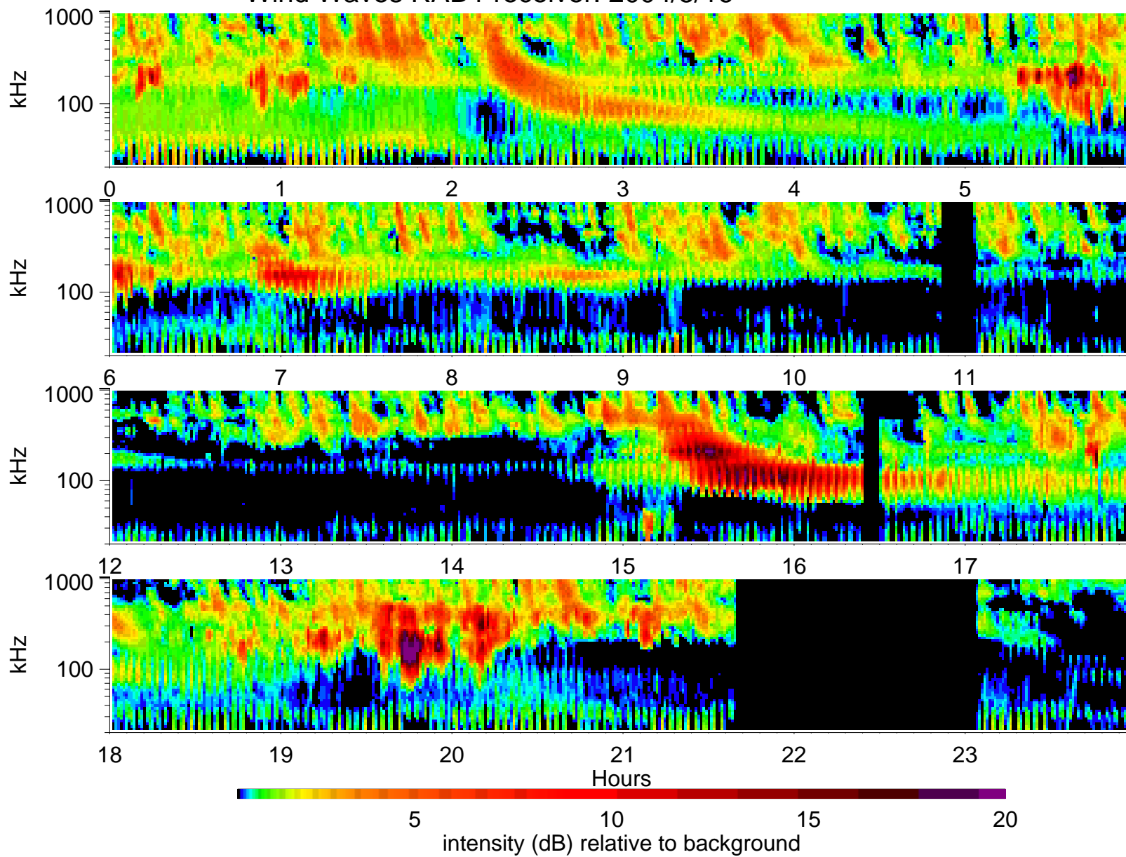
Wind Waves RAD1 receiver: 2004/5/16
