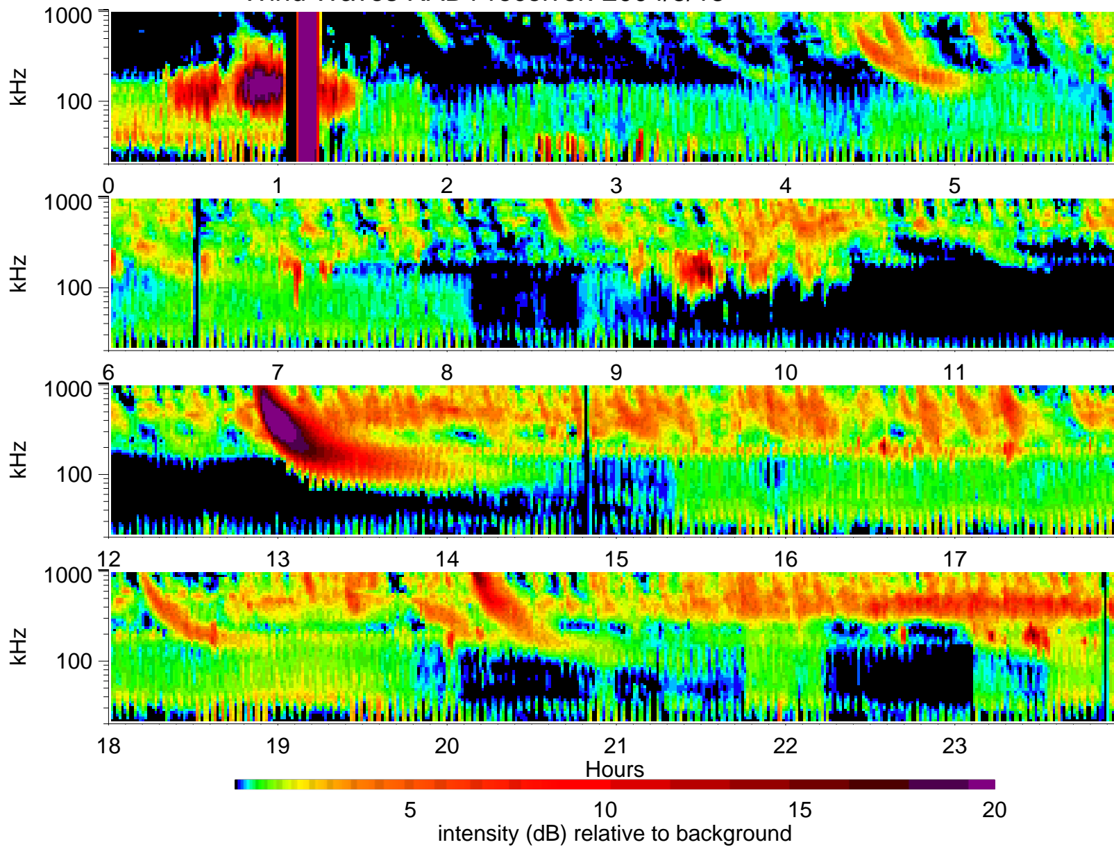
Wind Waves RAD1 receiver: 2004/5/15
