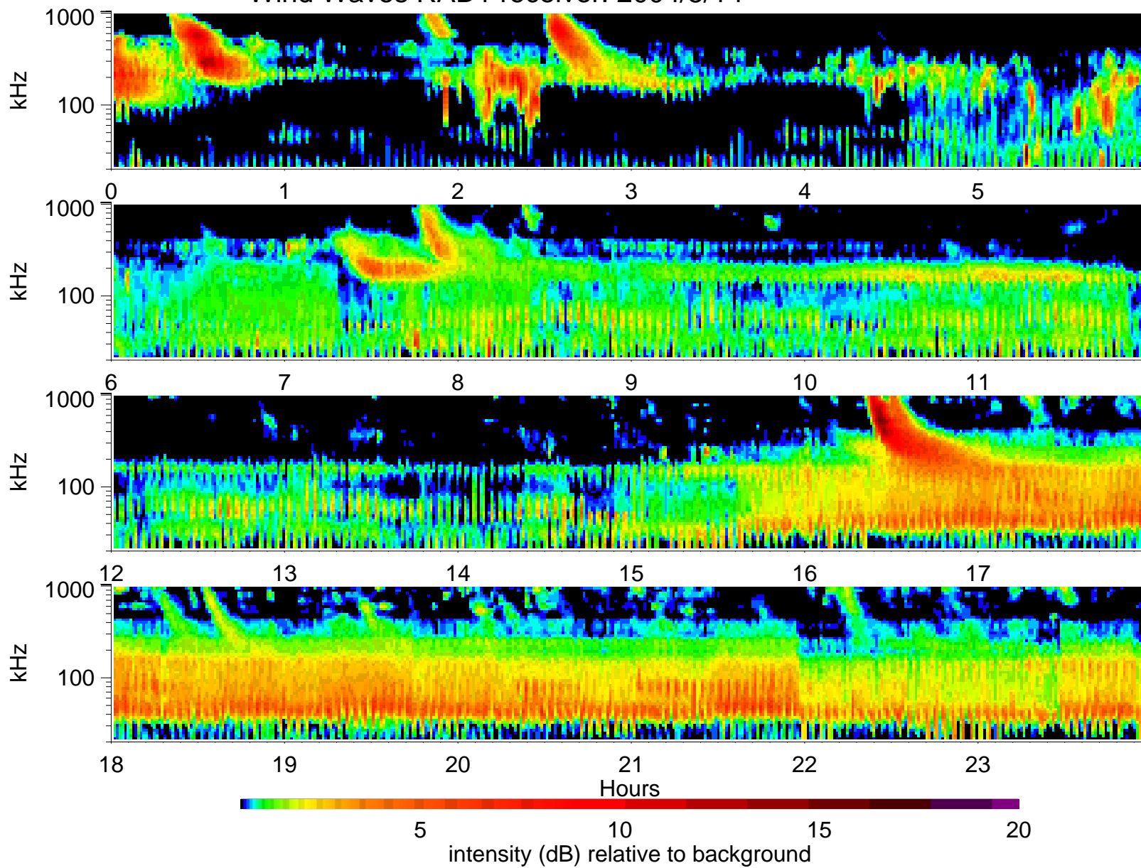
Wind Waves RAD1 receiver: 2004/5/14
