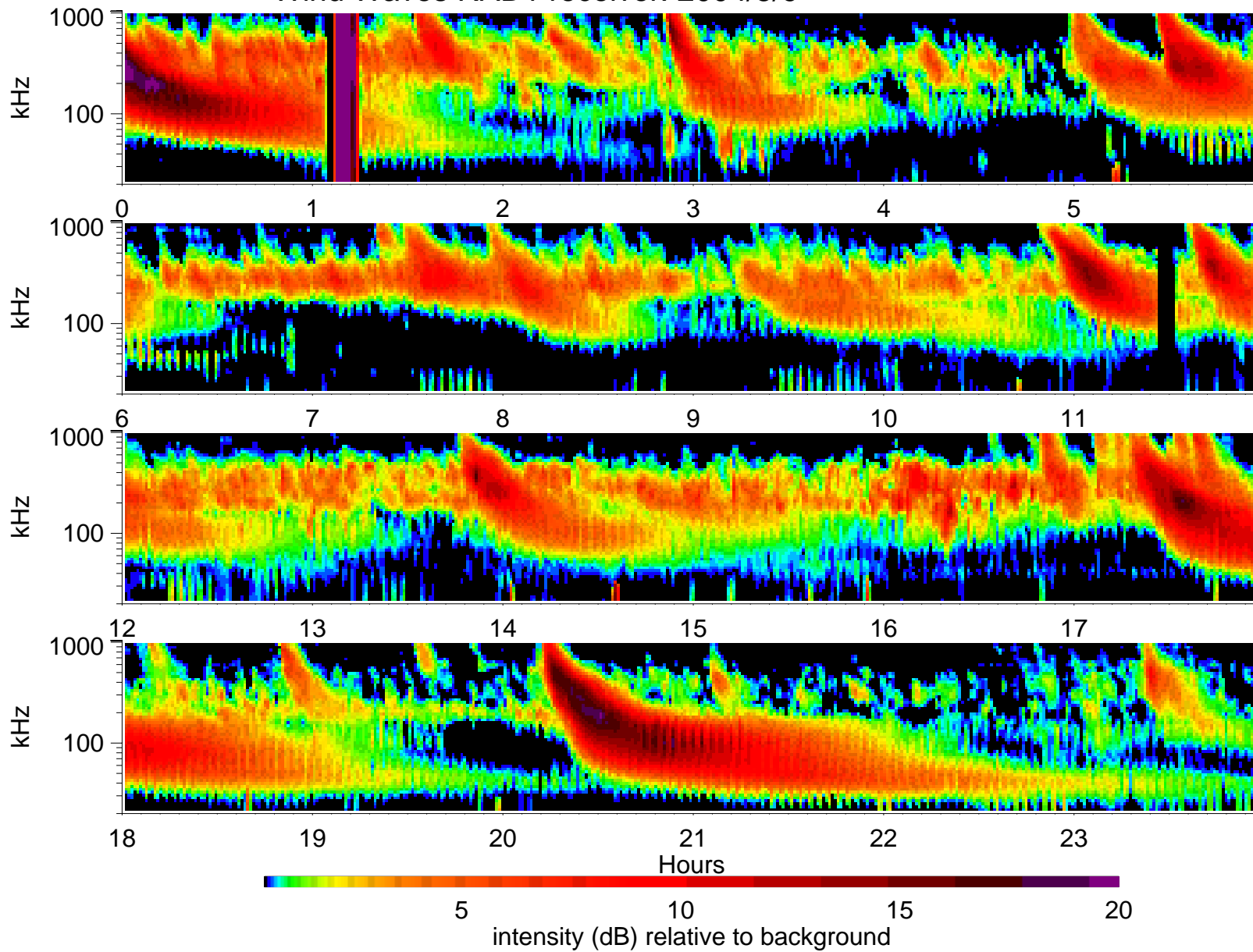
Wind Waves RAD1 receiver: 2004/5/9
