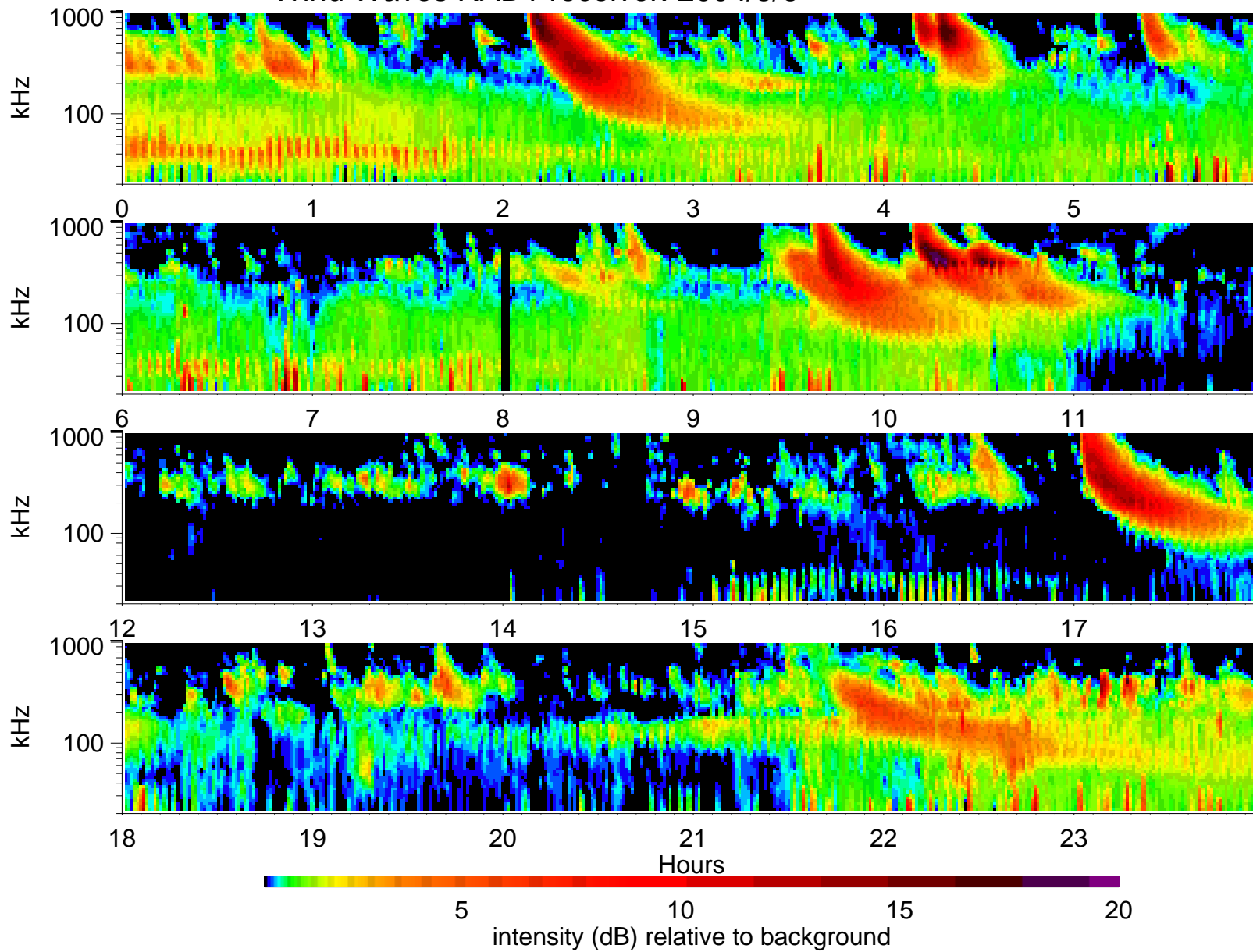
Wind Waves RAD1 receiver: 2004/5/6
