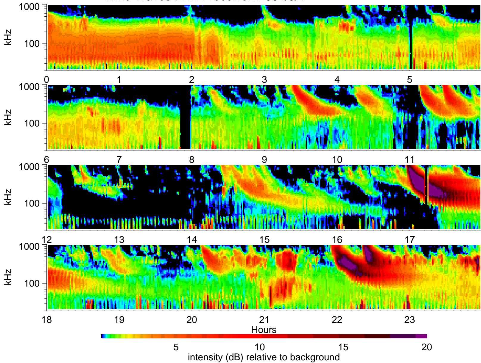
Wind Waves RAD1 receiver: 2004/5/4
