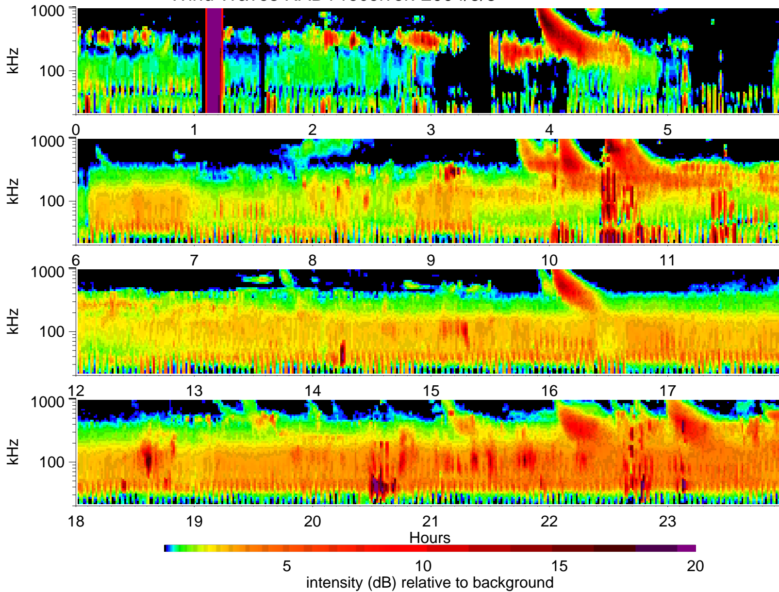
Wind Waves RAD1 receiver: 2004/5/3
