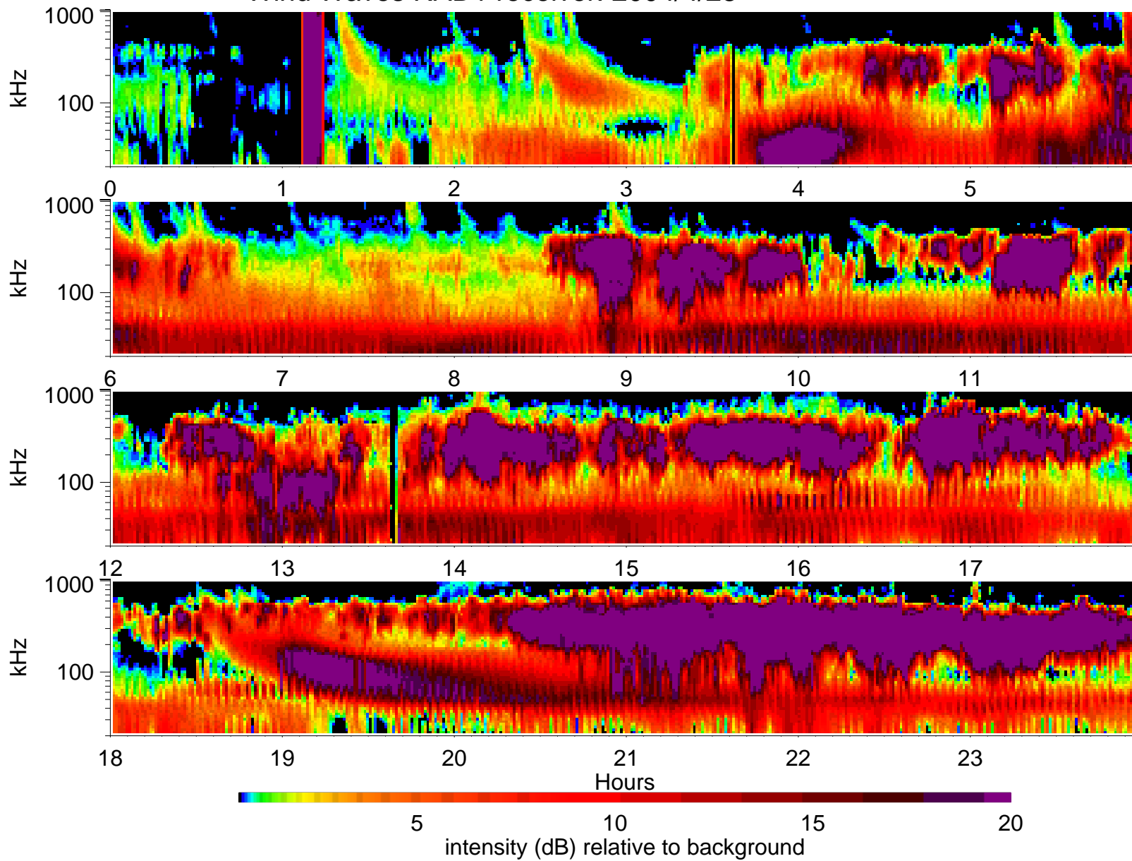
Wind Waves RAD1 receiver: 2004/4/23
