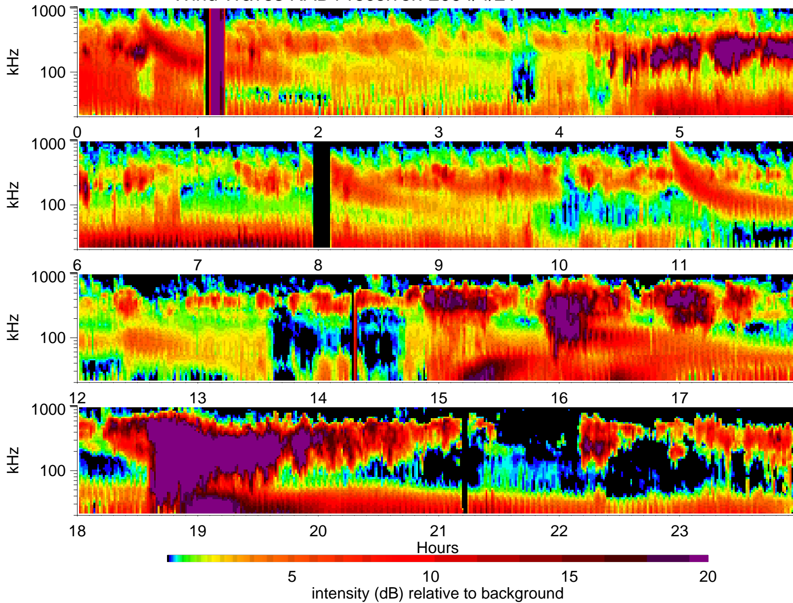
Wind Waves RAD1 receiver: 2004/4/21
