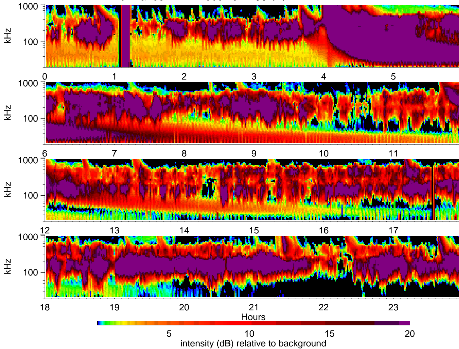
Wind Waves RAD1 receiver: 2004/4/11
