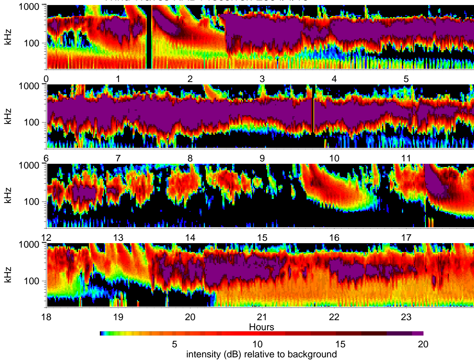
Wind Waves RAD1 receiver: 2004/4/10
