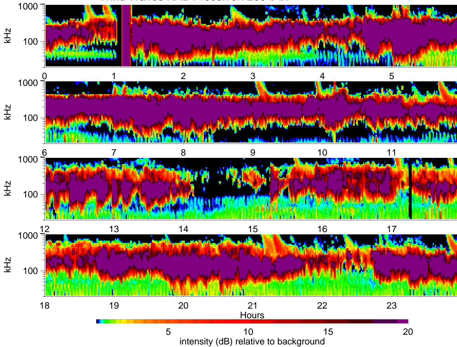
Wind Waves RAD1 receiver: 2004/4/7
