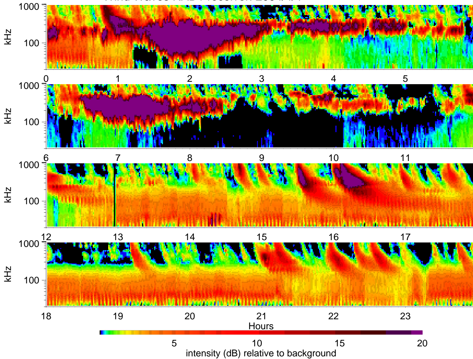
Wind Waves RAD1 receiver: 2004/4/4
