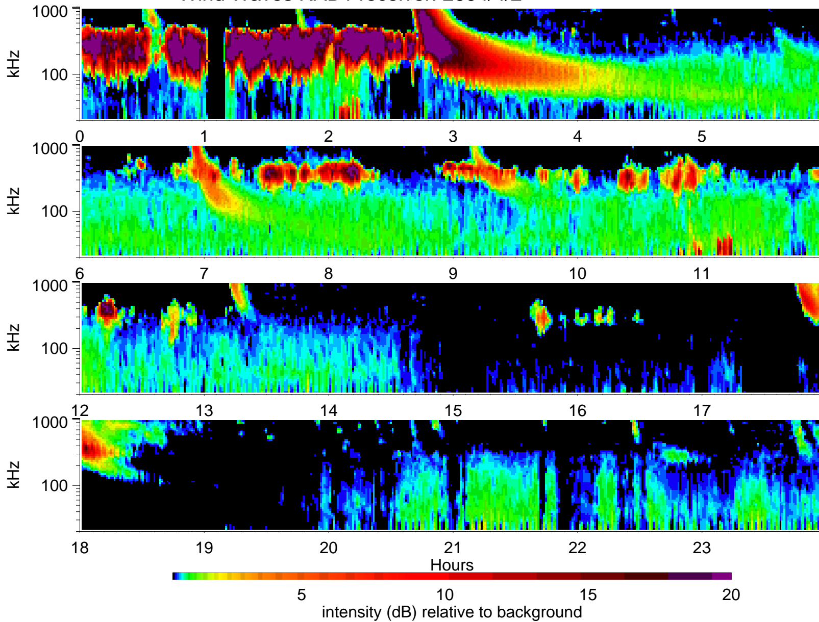
Wind Waves RAD1 receiver: 2004/4/2
