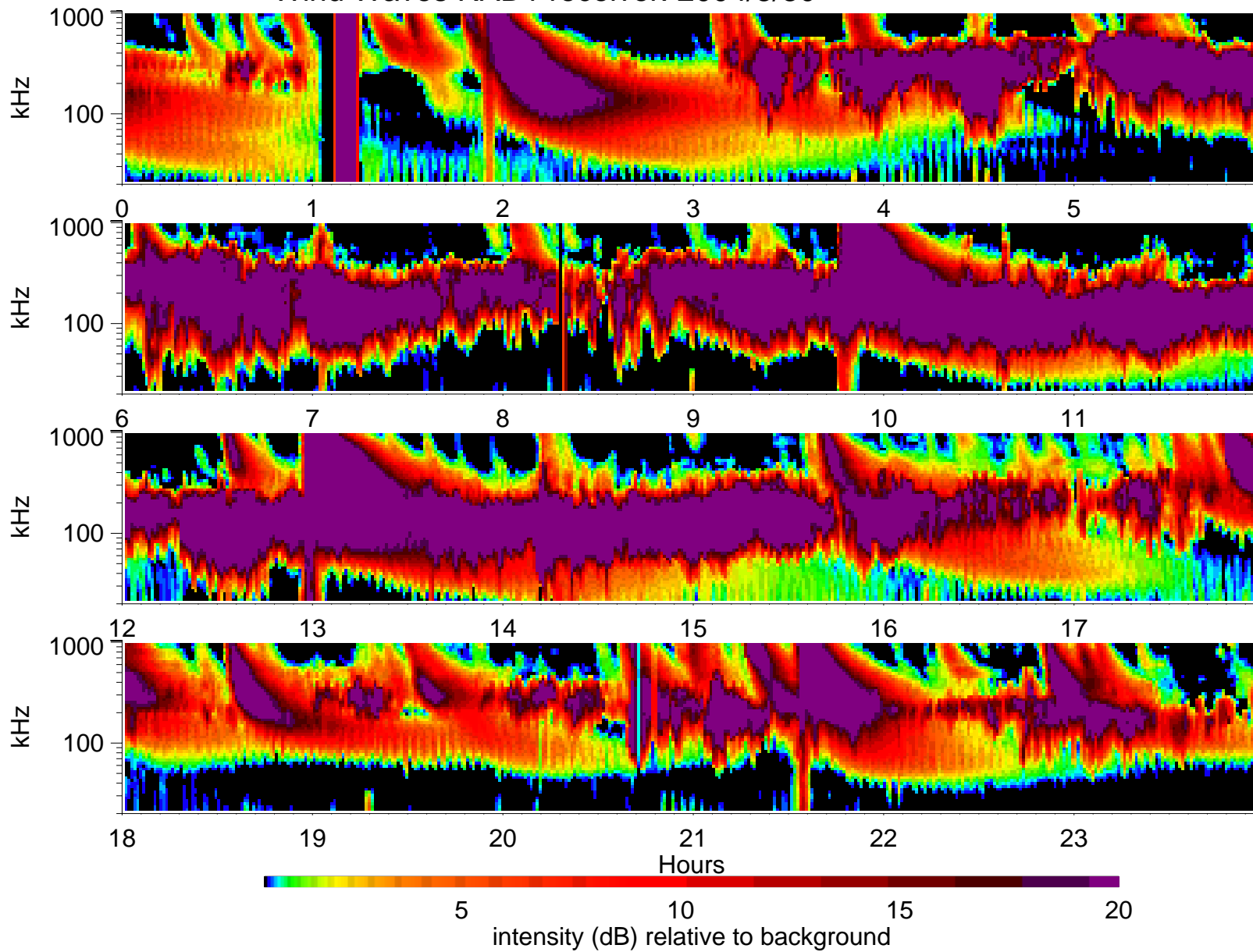
Wind Waves RAD1 receiver: 2004/3/30
