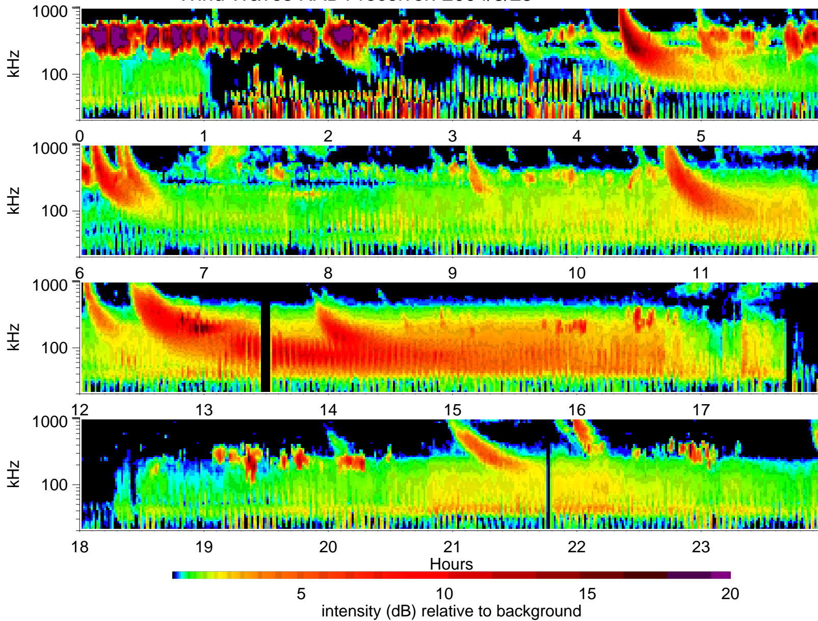
Wind Waves RAD1 receiver: 2004/3/25
