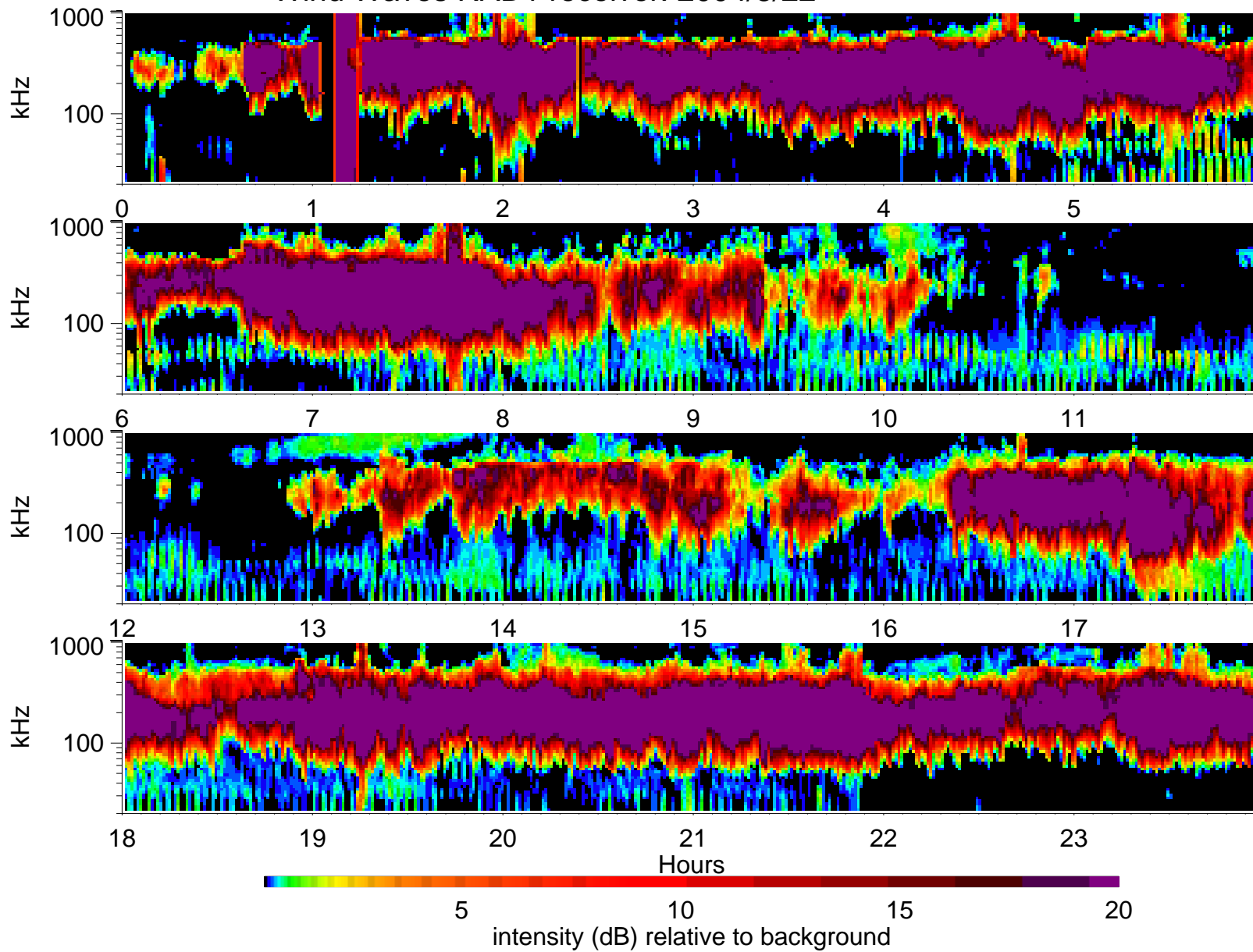
Wind Waves RAD1 receiver: 2004/3/22
