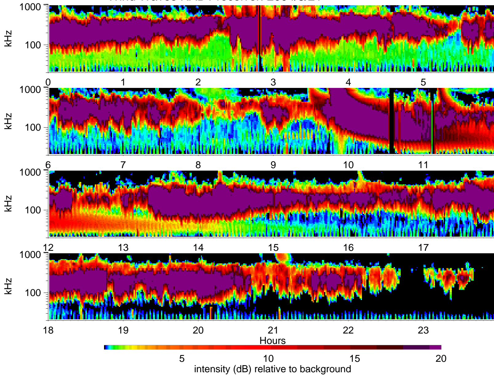
Wind Waves RAD1 receiver: 2004/3/21
