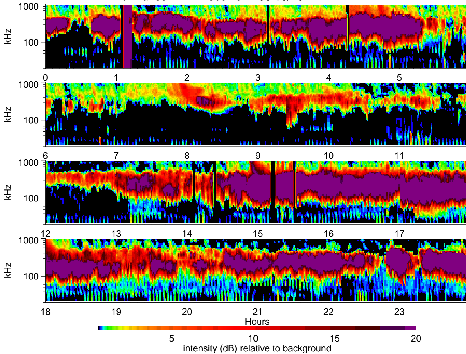
Wind Waves RAD1 receiver: 2004/3/20
